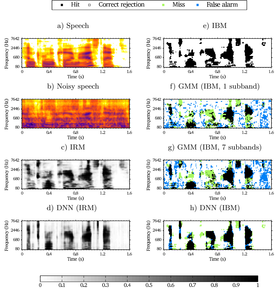
Figure 3.3: Estimated and ideal time-frequency masks for an CLUE sentence mixed with ICRA7 noise at -5 dB SNR. The spectrograms of clean and noisy speech are shown in Figs. 3.3a and 3.3b. The IRM and the IBM are shown in Figs. 3.3c and 3.3e. A selection of estimated masks from system configurations are shown in Figs. 3.3d, 3.3f, 3.3g and 3.3h. Misses (speech-dominated T-F units erroneously labeled as noise-dominated) and false alarms (noise-dominated T-F units erroneously labeled as speech-dominated) are shown on top of the estimated IBMs. The estimated IBM in Fig. 3.3h was converted from the corresponding estimated IRM by applying a threshold, which was derived from Eq. (3.1) at -5 dB SNR and using \beta = 0.5 .
